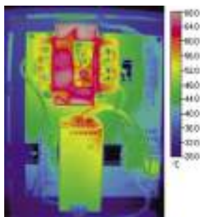
Allen-Bradley 1606-XLS – 10 A, 24V DC – 93% Efficiency
