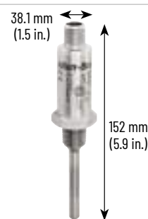
837T Non-Display Temperature Sensors
