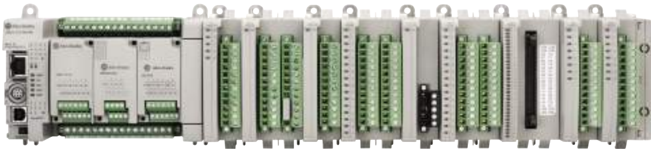
Micro870 Controller with Expansion I/O Modules
